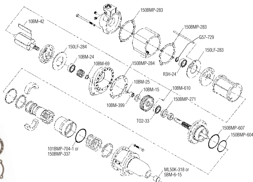
Exploded View of 150BM-TK2 Part Location
