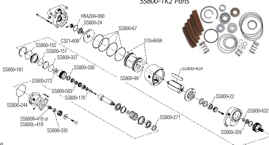
Exploded View of SS800-TK2 Part Location
