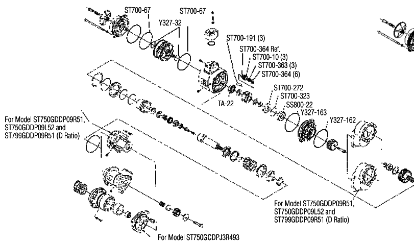
Exploded View of ST700-TK1 Part Location
