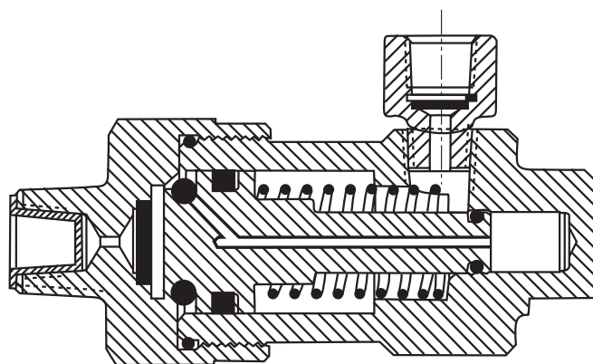
HDL2/HDL3 Cross Section
