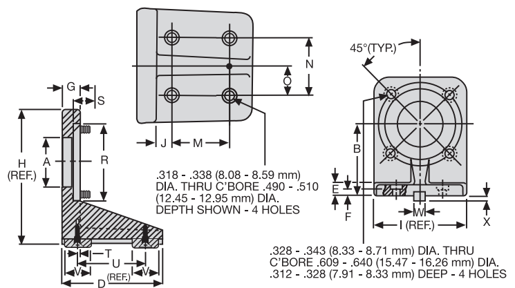
45090 FOOT MOUNTING BRACKET
