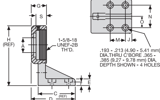
37894 FOOT MOUNTING BRACKET
