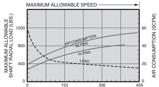
SPEED FOR DETERMINING SHAFT RADIAL LOAD
